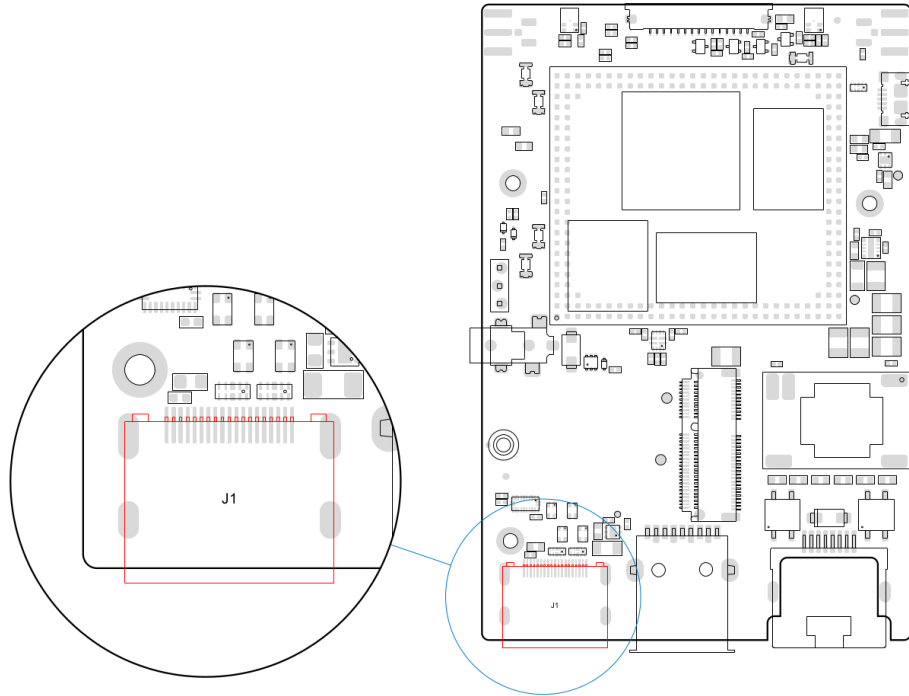
Figure 5: HDMI connector
