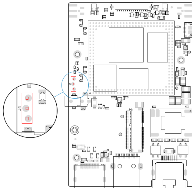
Figure 4: Debug port
