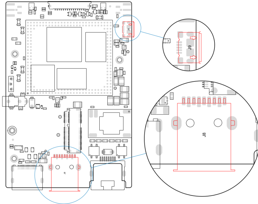
Figure 13: USB connectors
