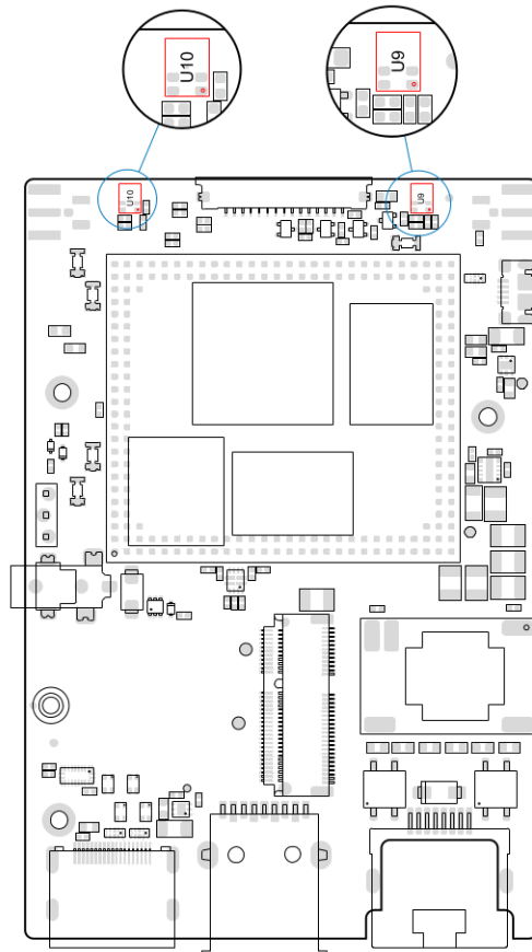
Figure 10: MEMS microphones
