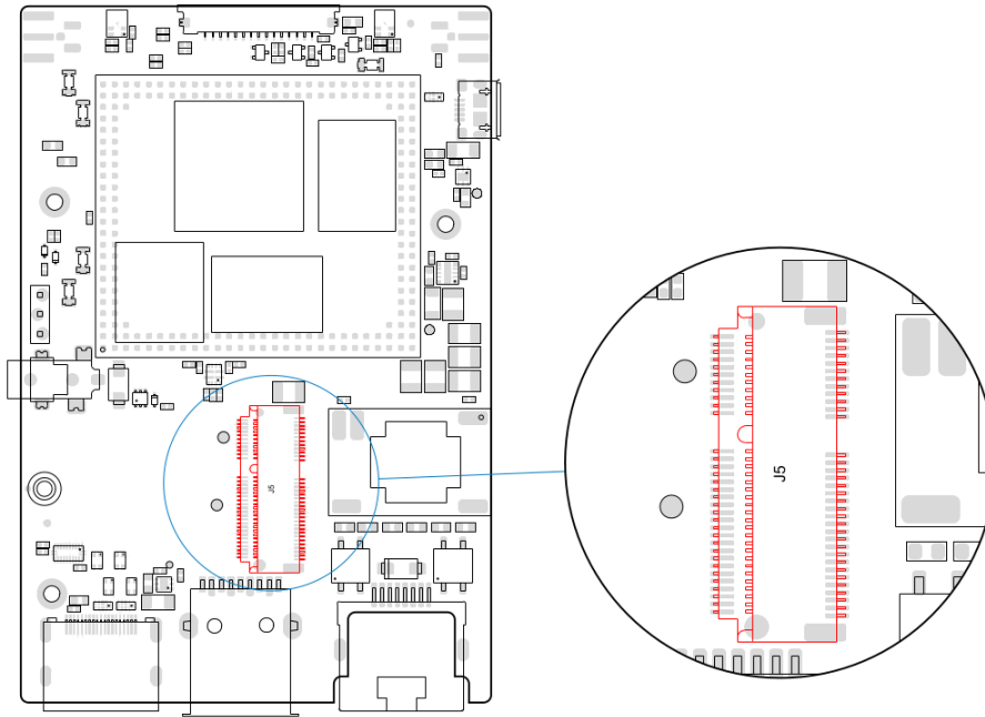
Figure 11: M.2 interface
